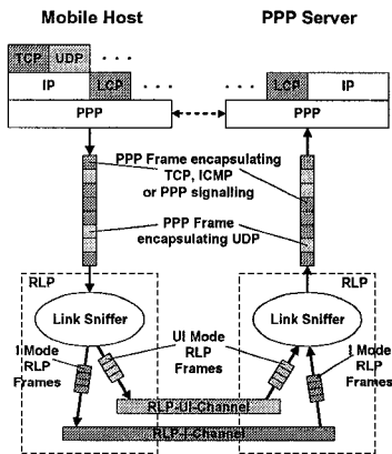
Fig. 7. Reliable and delay-sensitive data over RLP.
