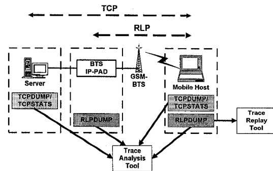
Fig. 9. The TCP/RLP trace collection platform.
