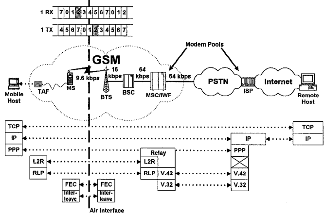
Fig. 1. TCP/IP over circuit-switched data in GSM.
