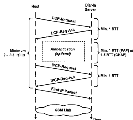
Fig. 5. PPP link configuration phase.
